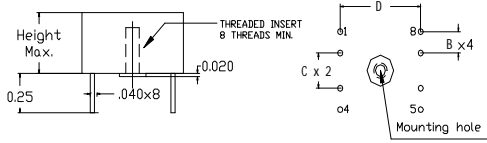
Suggested pcb layout
